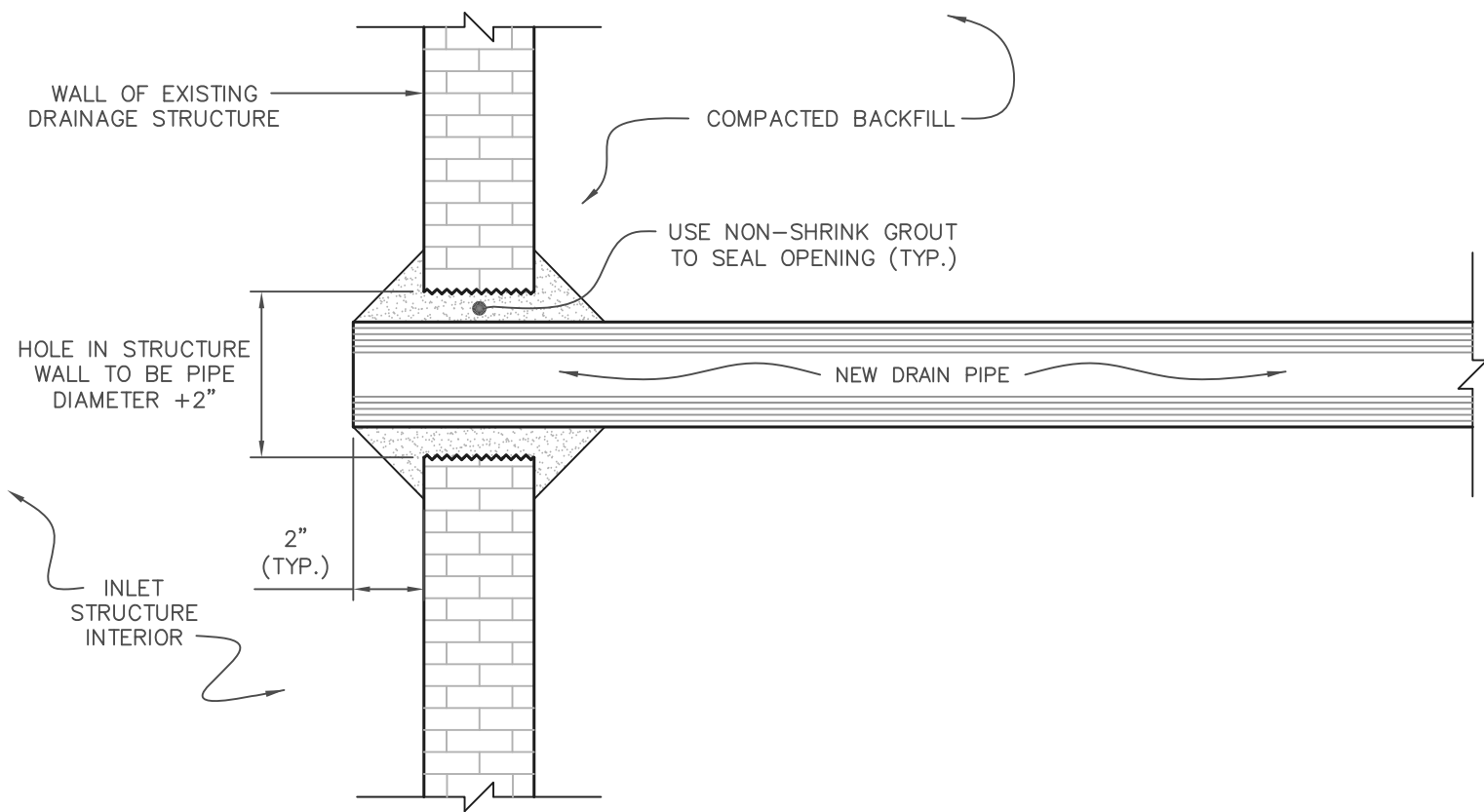
YARD DRAIN 'TIE-IN' DETAIL (TO EXISTING DRAINAGE STRUCTURE)
