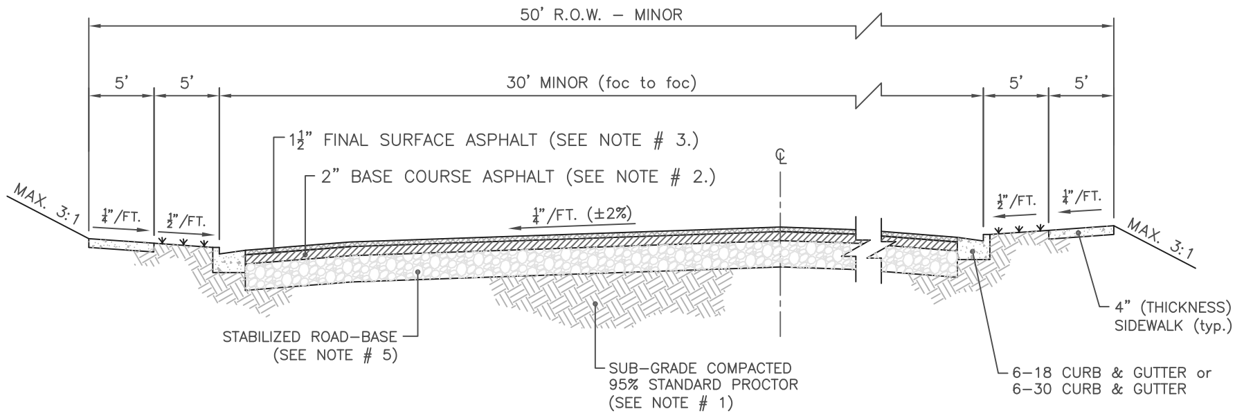
MINOR STREET TYPICAL SECTION
