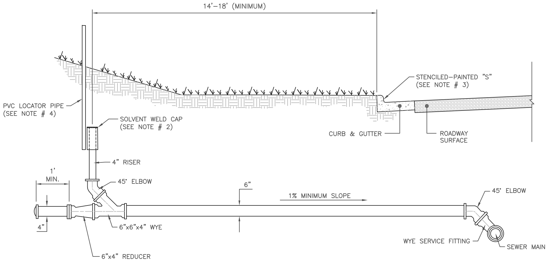
TYPICAL SEWER SERVICE CONNECTION
